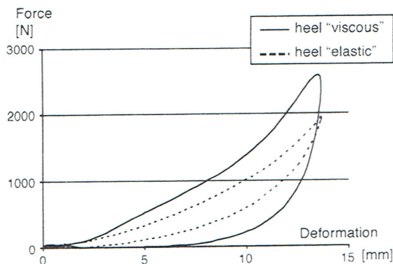
Fig. 1. Force–deformation diagrams for the two heels of the tested shoes as determined through MTS testing at 300 mm/s. Each curve is the average of three test results under the same conditions.
